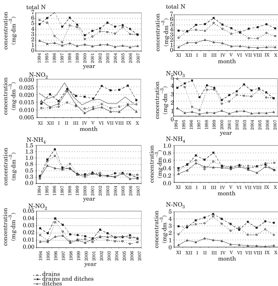
Fig. 5. Dynamics of the annual and monthly nitrogen concentrations in water discharged from agricultural areas in 1994-2007 ( \text{mg dm}^{-3} )
