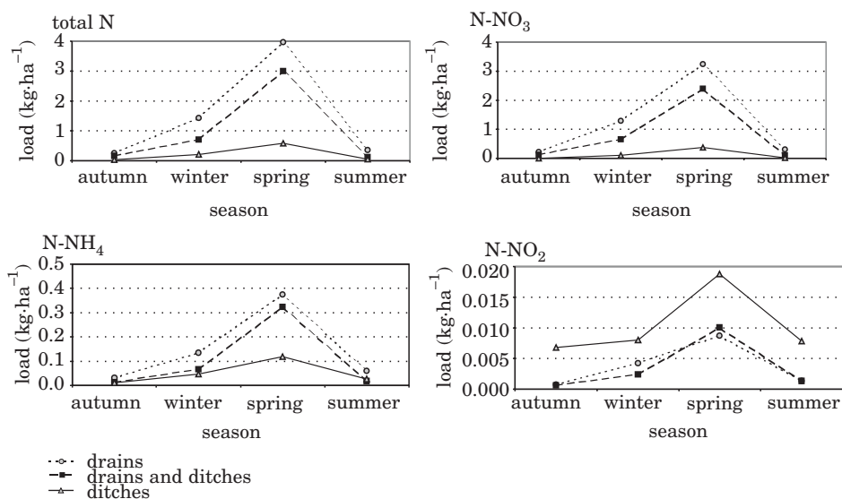
Fig. 10. Seasonal dynamics of nitrogen outflow through draining systems in 1994-2007 ( \text{kg ha}^{-1} )
