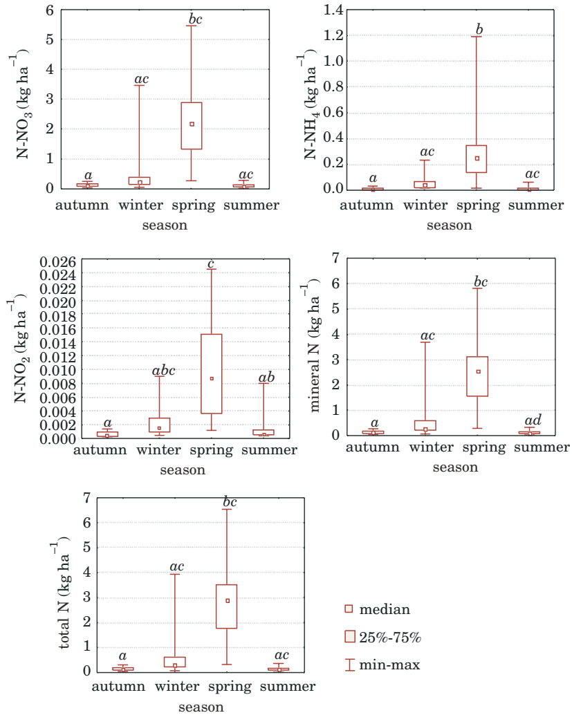
Fig. 12. Seasonal dynamics of loads of nitrogen in water discharged through a network of ditches and drains
