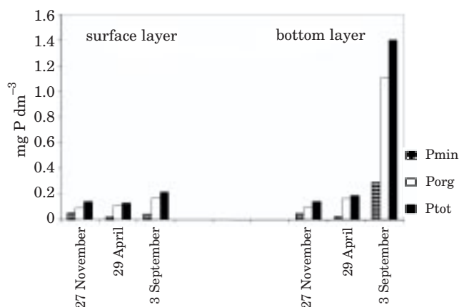
Fig. 3. Changes of phosphorus compounds content in waters of lake Gi³wa
