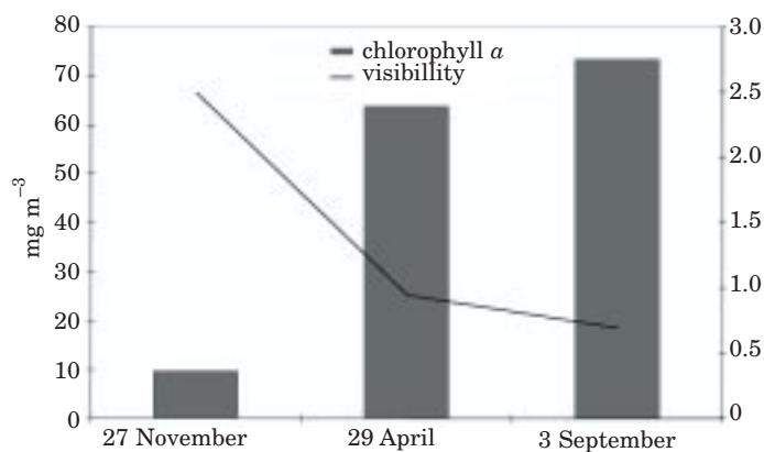
Fig. 2. Chlorophyll a content and visibility of Secchi disc in water of Lake Gi 3 wa
