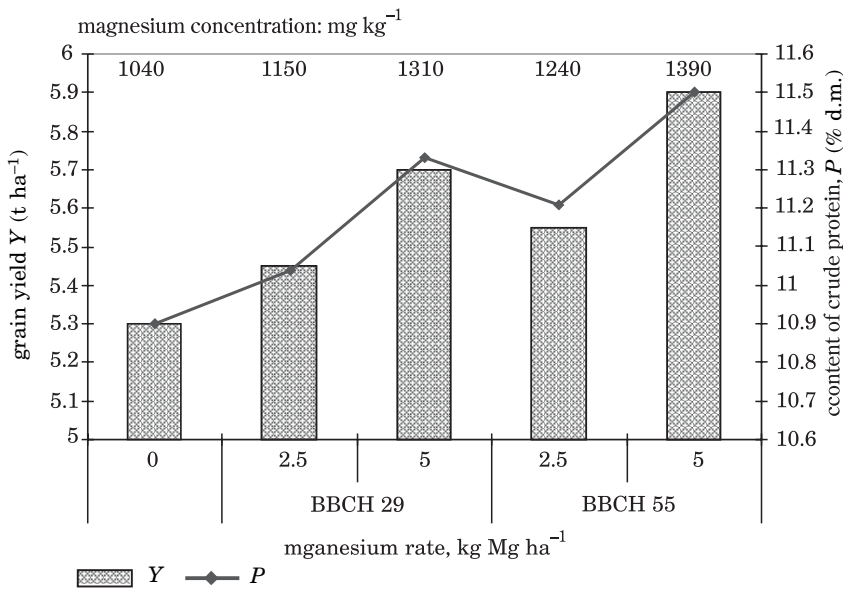
Fig. 8. Effect of timing and magnesium application rate on quantity and quality of winter wheat grain (based on MATŁOŚZ 1992)
